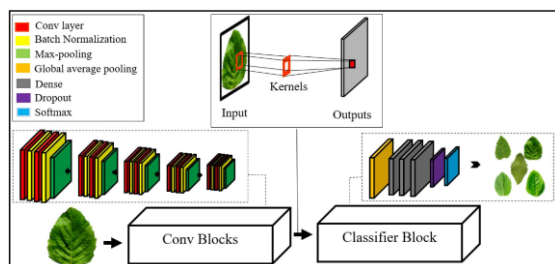
Figure 4 — Deep learning architecture
