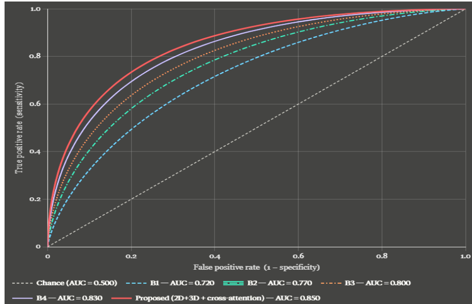
Figure 2: ROC curves for five models on the PPMI held out test set. x-axis: 1-Specificity. y-axis: Sensitivity negative scores \sim N(0,1) calibrated so each curve's area matches the listed AUC to \pm 0.001 .
