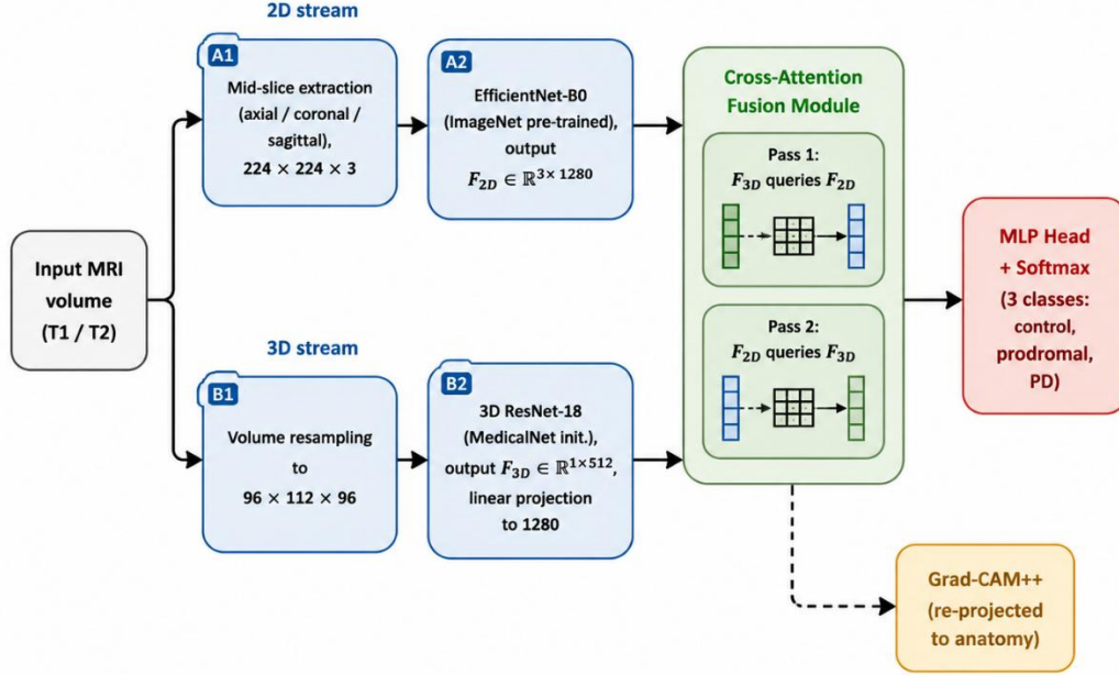
Figure 1: Hybrid 2D-3D deep learning architecture. EfficientNet-B0 encodes three planar mid-sections; 3D ResNet-18 encodes the full volume; a cross-attention block aligns the two representations before classification. Grad-CAM++ provides post-hoc anatomical attribution
