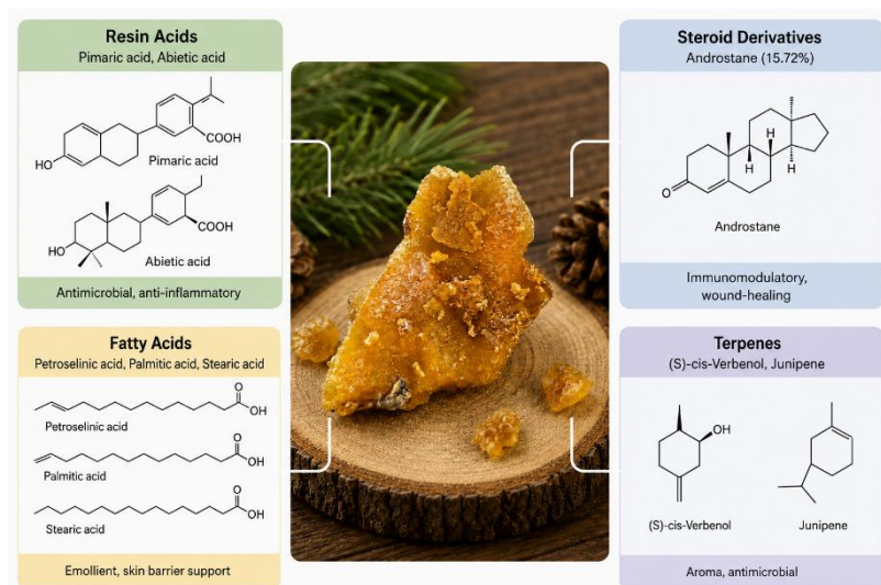
Figure 2. Results of the pine resin sample
