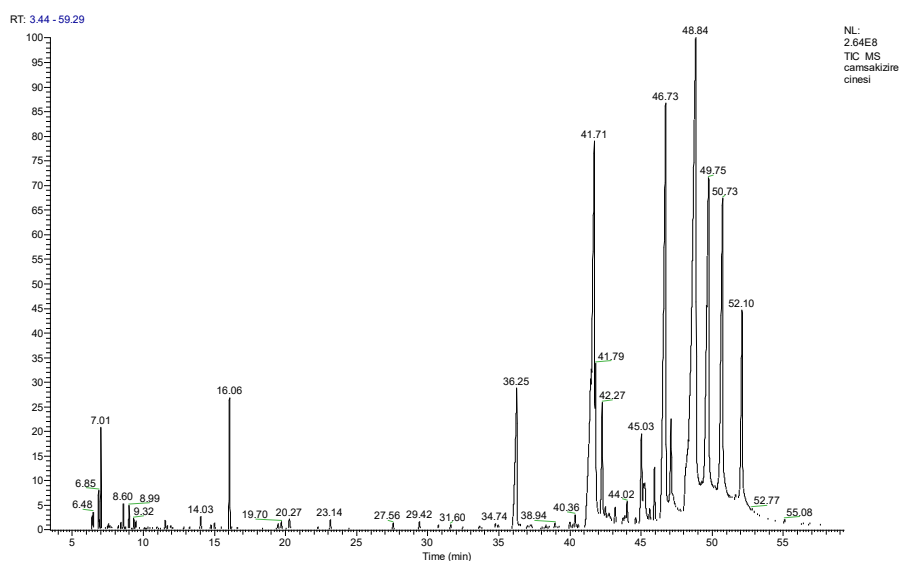
Figure 1. GC-MS chromatogram of the pine resin sample
