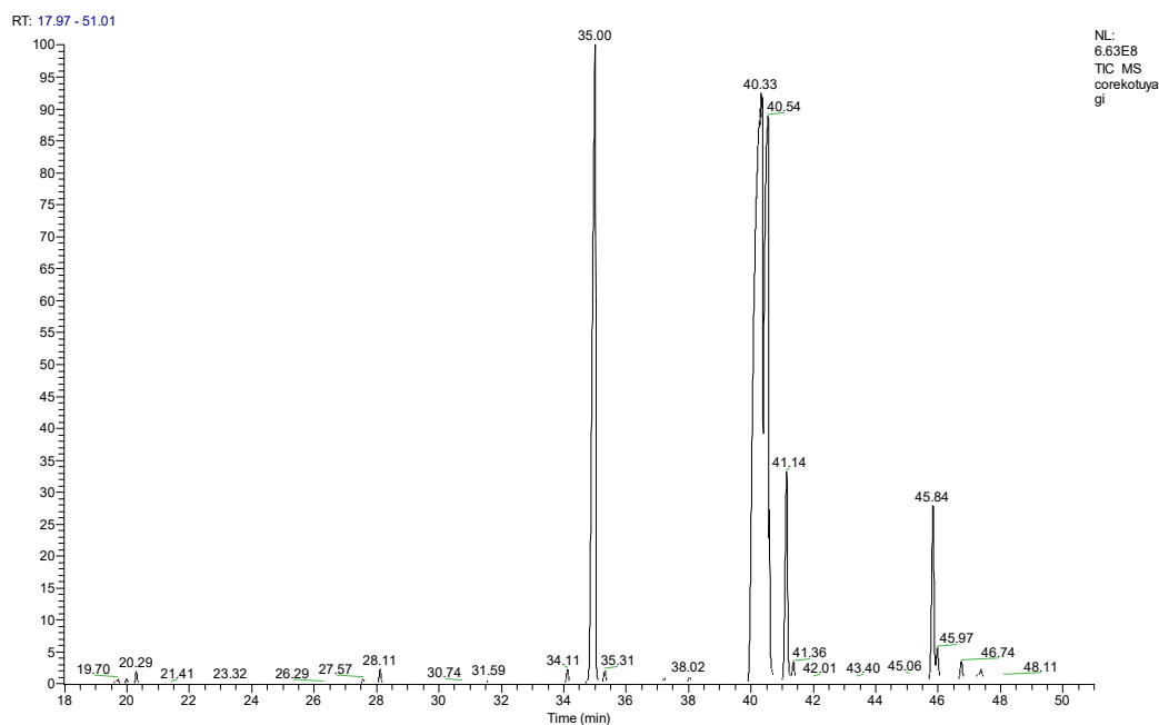
Figure 2. GC-MS chromatogram of the hexane extract of cold press Nigella sativa residue
