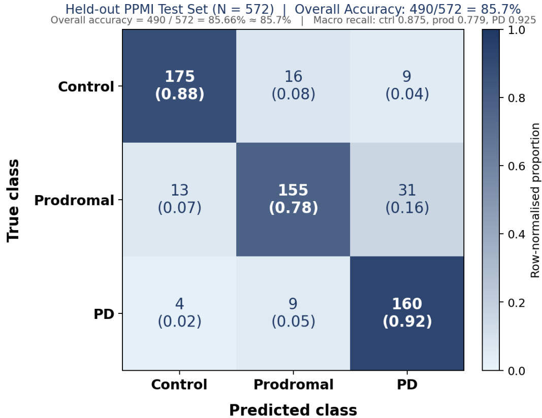
Figure 3: Confusion Matrix on the held-out PPMI test set for the proposed hybrid model
