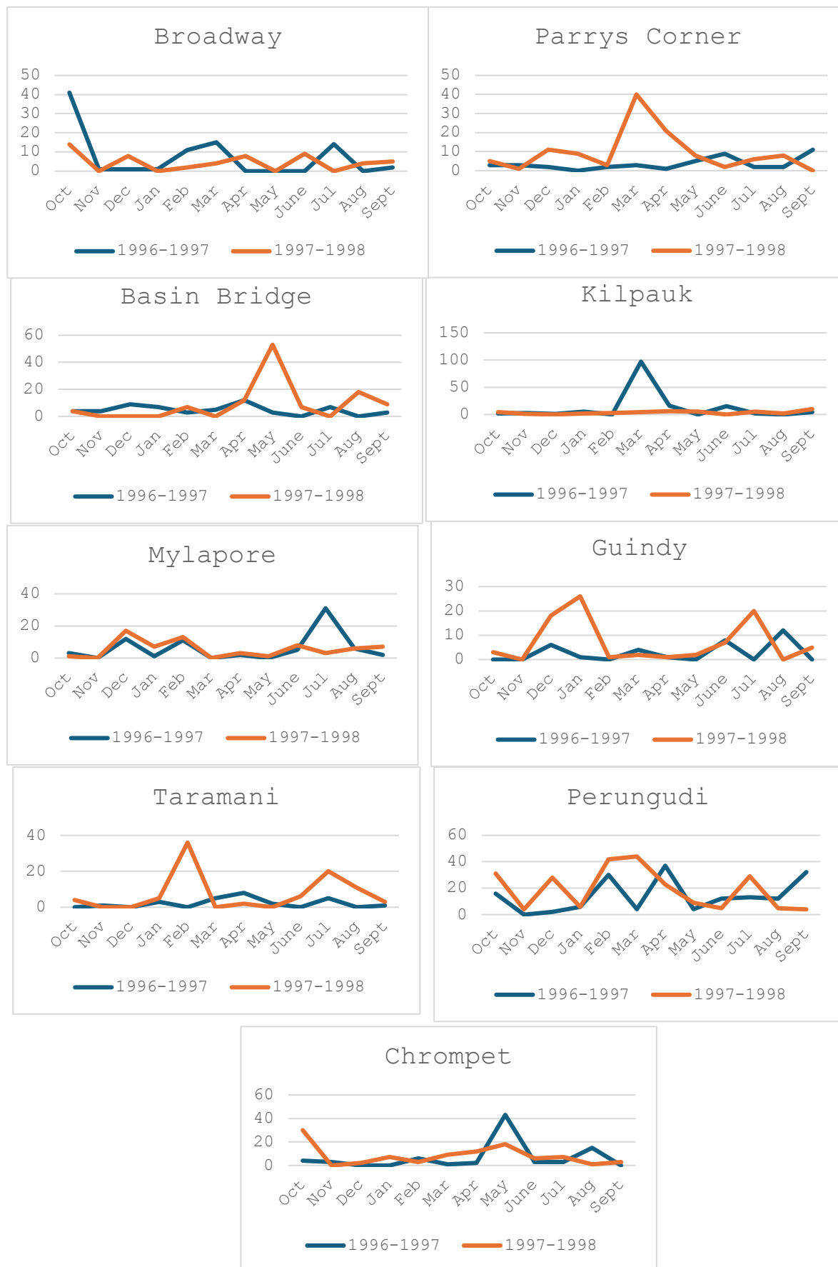
Fig. 3. Seasonal Distribution of the fungus, Aspergillus fumigatus in the atmosphere of different sampling sites in Chennai during October 1996 to September 1998.
