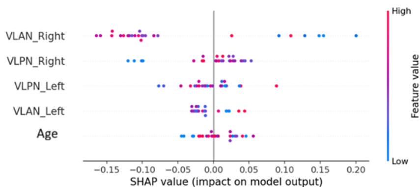
Figure 5. SHAP results
