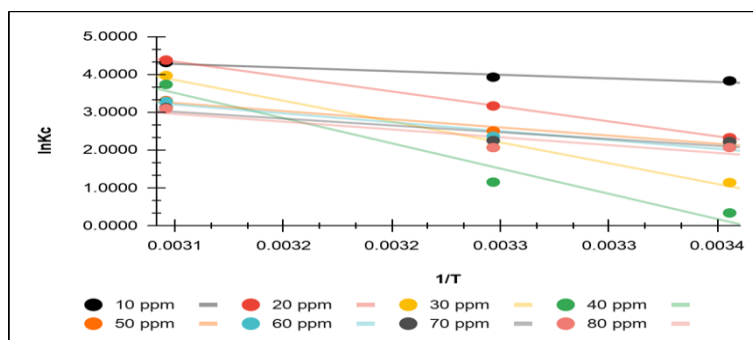
Figure 7. Thermodynamic graphs plotted for Crystal Violet dye on Van/Erciş soil
