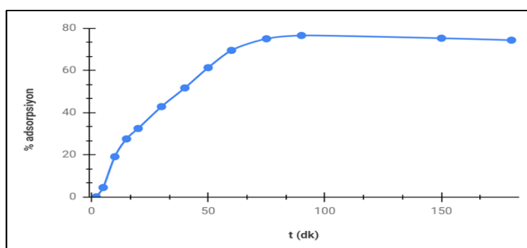
Figure 2. Adsorption plot of crystal violet dye as a function of time (m: 0.1 g, V: 0.05 ml, C 0 : 20 ppm, T: 298 K).
