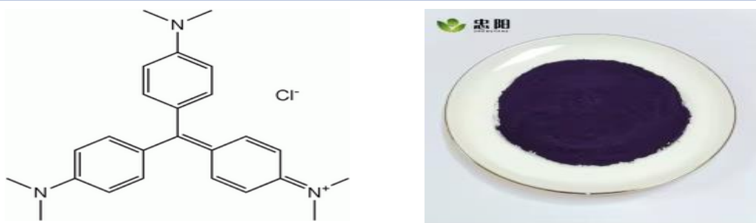
Figure 1. The formula (C 25 H 30 ClN 3 ) and structure of crystal violet (Mittal et al., 2010).
