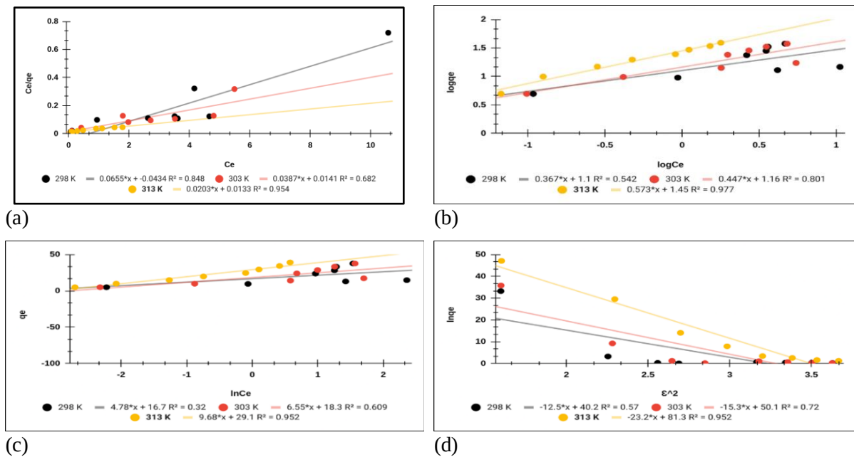
Figure 6. Langmuir (a), Freundlich (b), Temkin (c) and D-R (d) isotherm plots for Crystal Violet dye on Van/Erciş soil.
