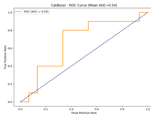
Figure 2. ROC Curve of the CatBoost Model
