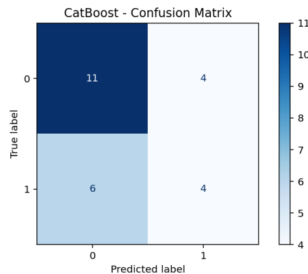
Figure 3. Confusion Matrix for CatBoost Model
