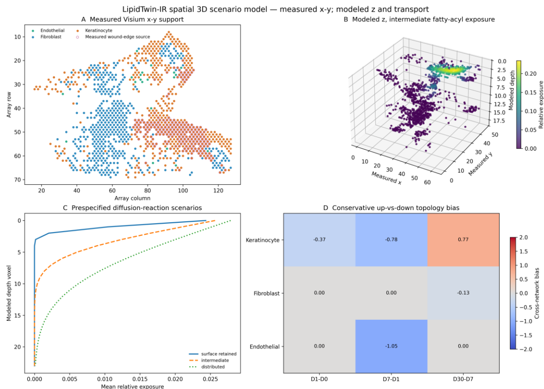
Figure 6 | Measured-x-y/modelled-z spatial 3D scenario model.
