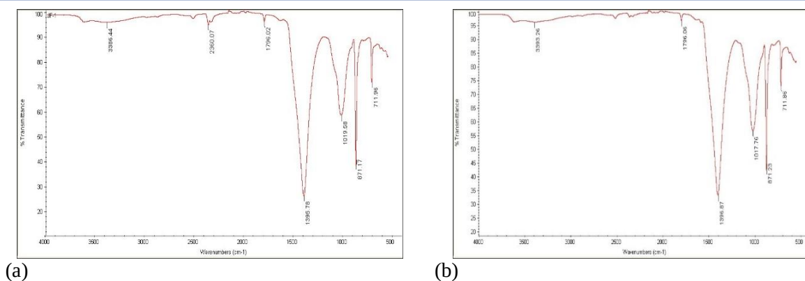
Figure 5. FTIR spectrum images of soil (a) and soil with KV adsorbed (b) samples.
