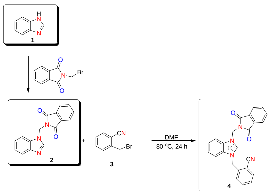
Figure 1. Synthesis of compound 4.
